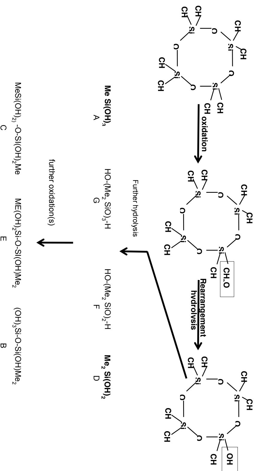
Figure 1 : Adapted from Varaparth et al. (1999) – Possible pathways for formation of D_4 metabolites in rat urine.
